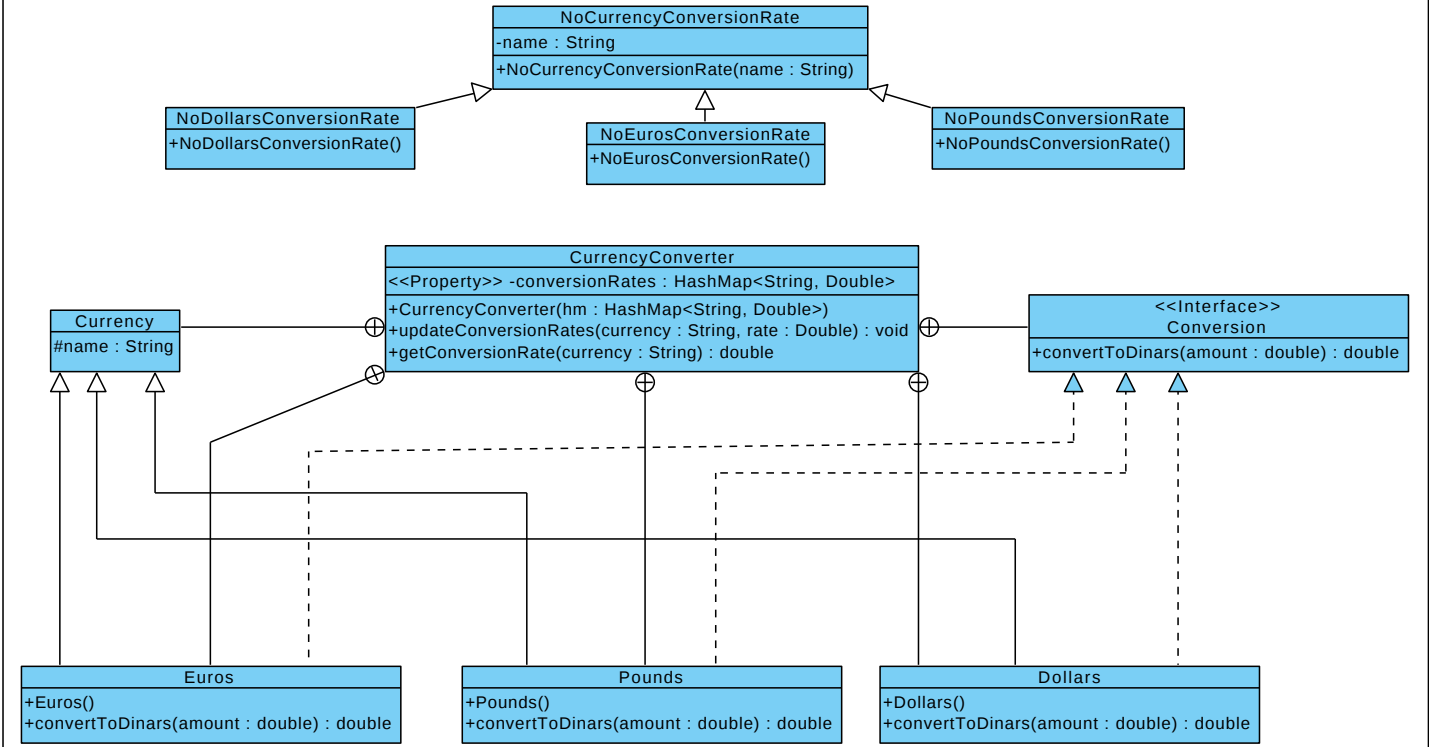
Class Diagram1
